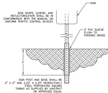
Sign Base Detail NTS
