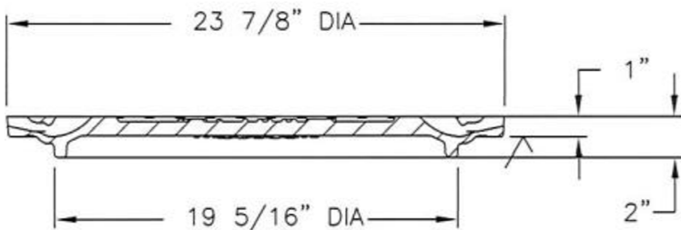
SECTION
