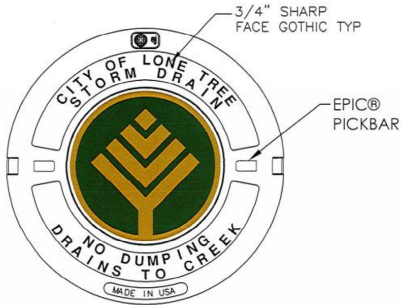
COVER FACE
