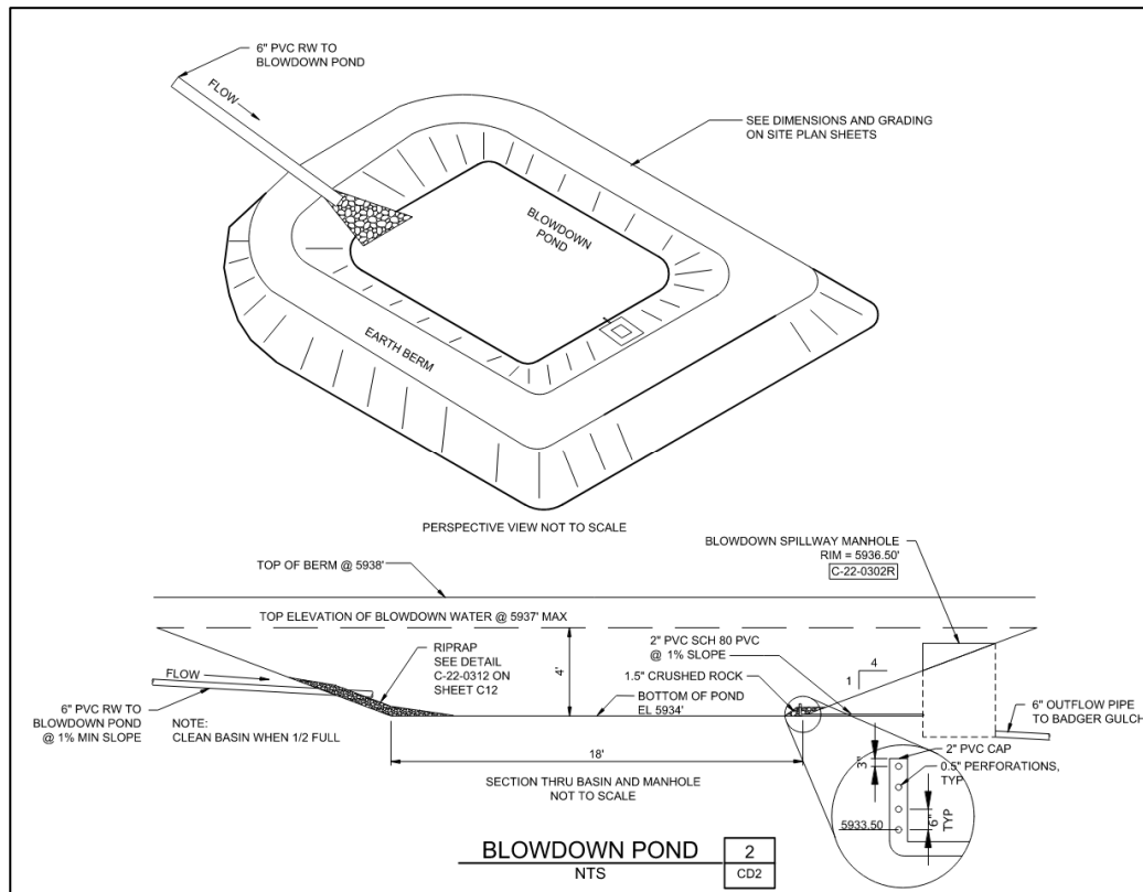
Figure 2: Blowdown Pond Detail
